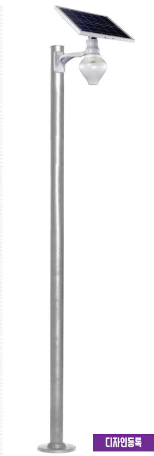
S701 Ø195×D605×H3000 LED 6W, 10W, 18W
